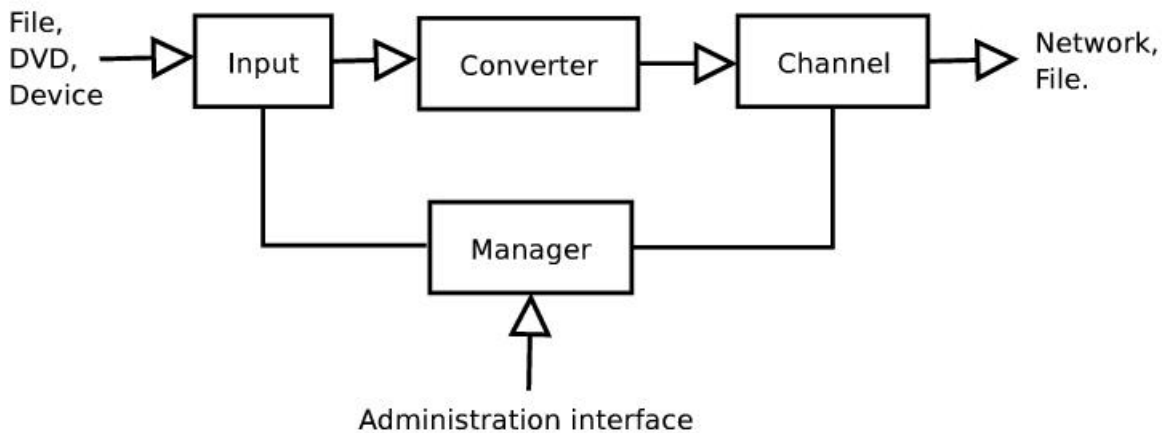
Figure 3-1. VLS structure
